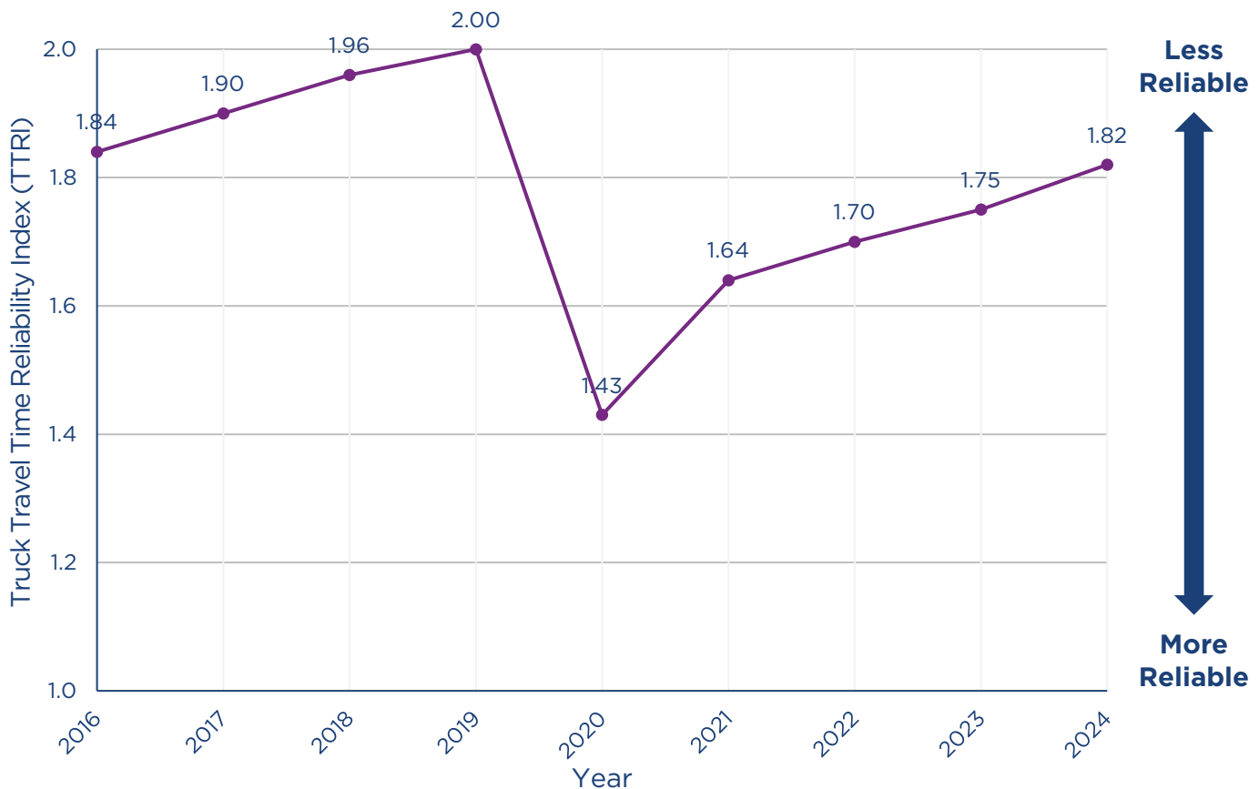
Truck Travel Time Reliability on Interstate Highways
